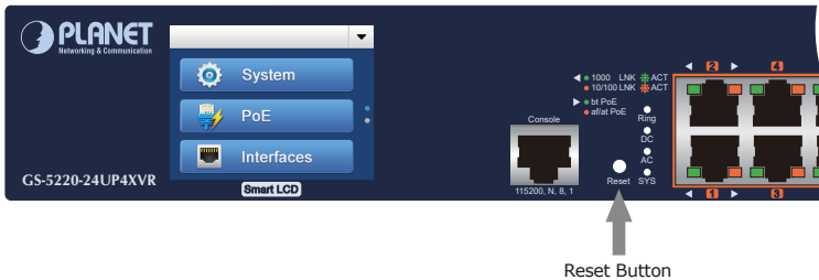
Figure 5-1: GS-5220 LCD Series Reset Button
